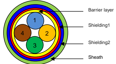
Insulation colors 1. Blue / White (Blue), 2. Orange / White (Orange) 3. Green / White (Green), 4. Brown / White (Brown)
